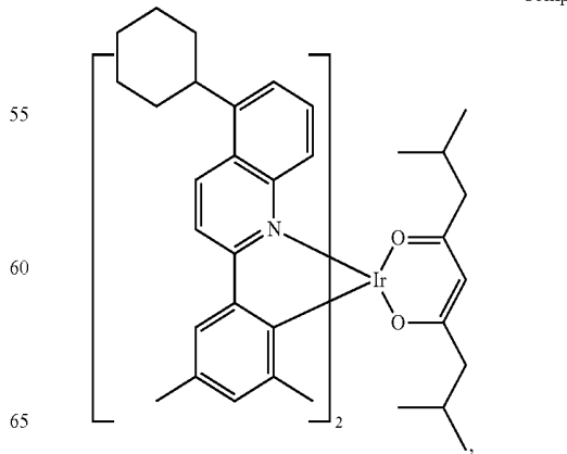
Compound II-11
