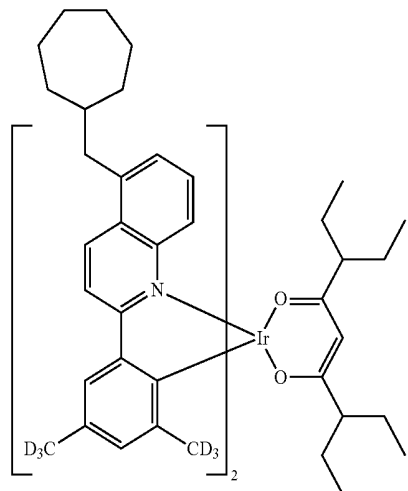
Compound II-68
