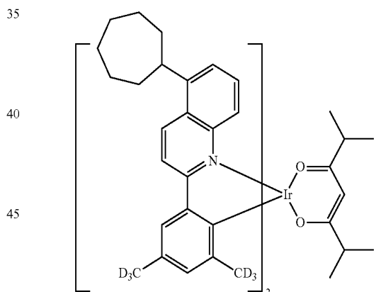
Compound II-44
