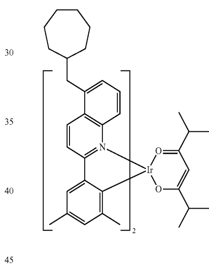
Compound II-21
