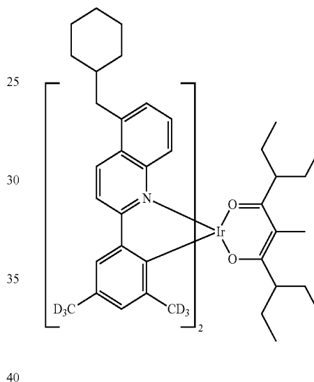
Compound II-68
