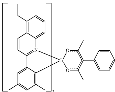
Compound 25
