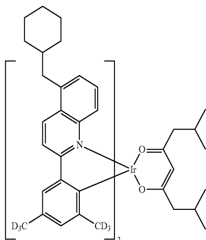
Compound II-63
