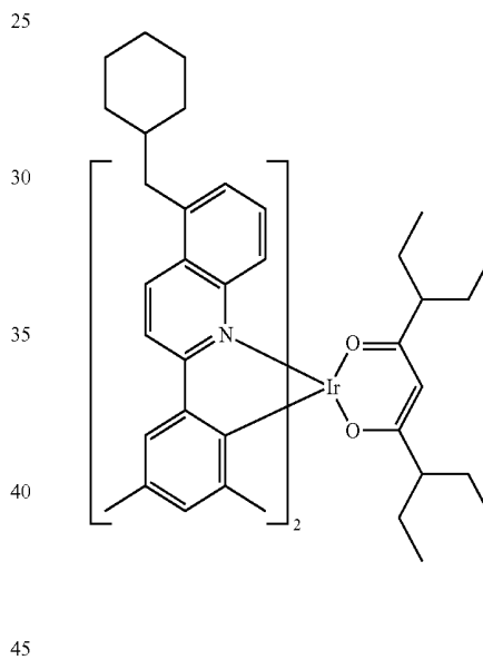
Compound II-31
