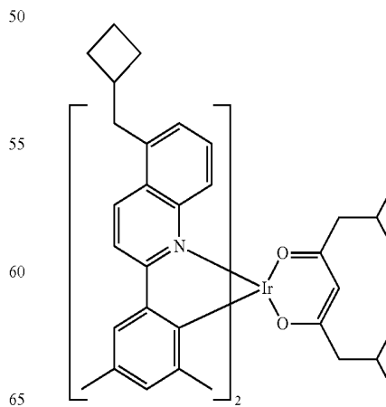
Compound II-25
