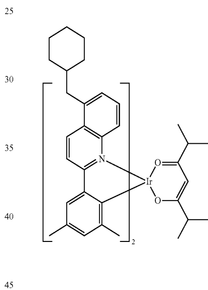
Compound II-20
