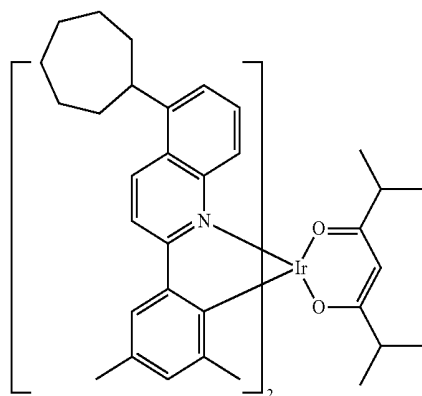
Compound II-8
