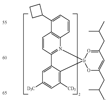
Compound II-41
