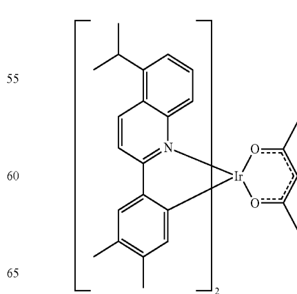
Compound 40
