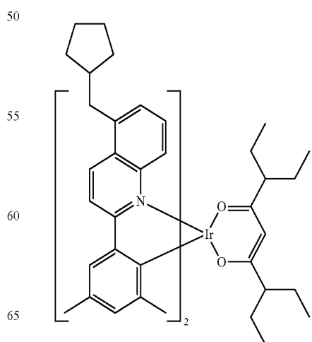
Compound II-30
