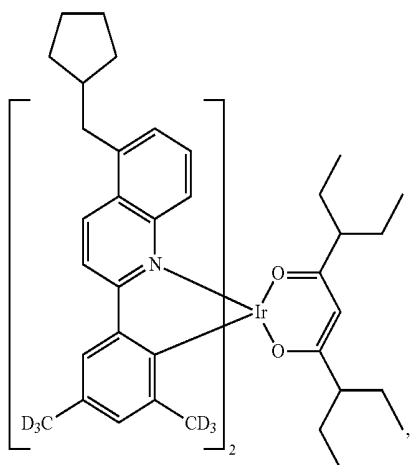
Compound II-66
