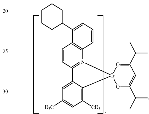
Compound II-44
