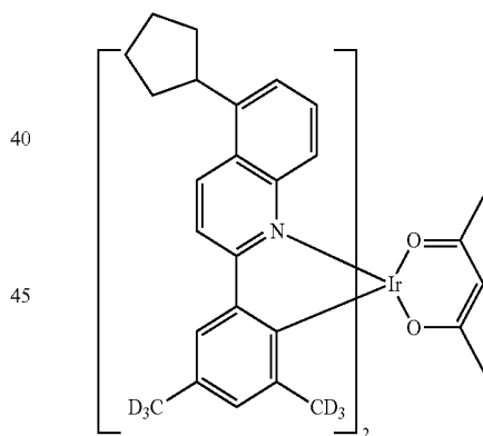
Compound II-35
