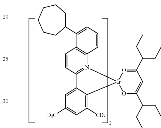
Compound II-51
