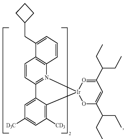
Compound II-65
