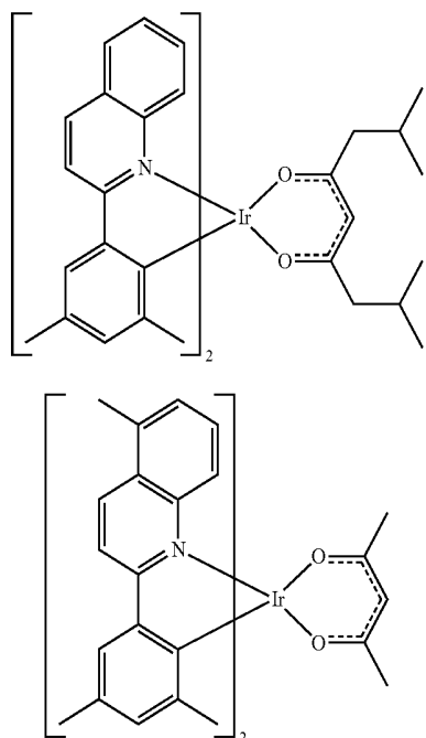
Compound D
