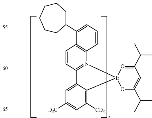
Compound II-44
