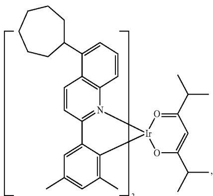
Compound II-8
