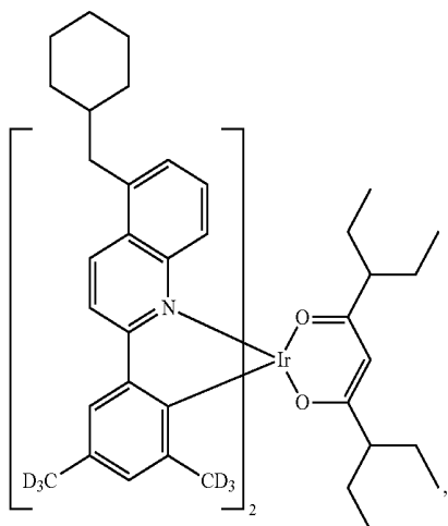
Compound II-67
