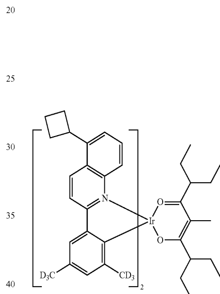
Compound II-48
