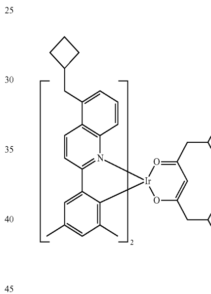
Compound II-22
