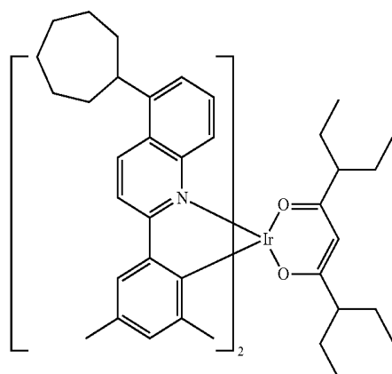
Compound II-16
