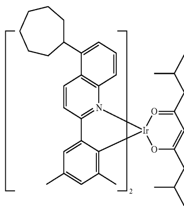
Compound II-8
