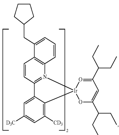
Compound II-66
