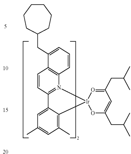
Compound II-25
