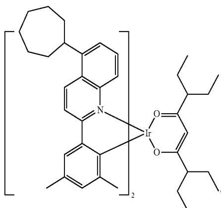
Compound II-16
