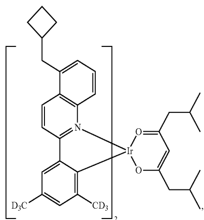
Compound II-61
