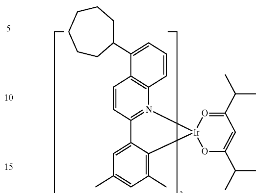
Compound II-9
