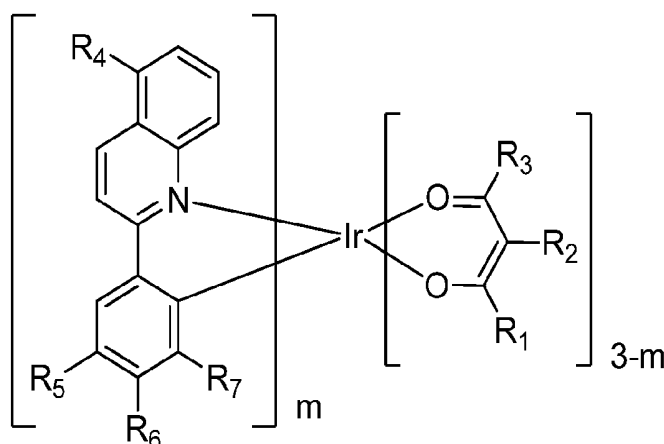
Formula III
