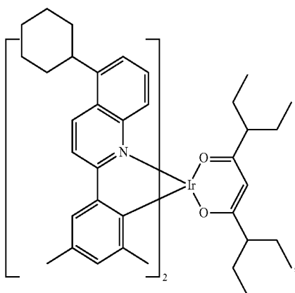
Compound II-15
