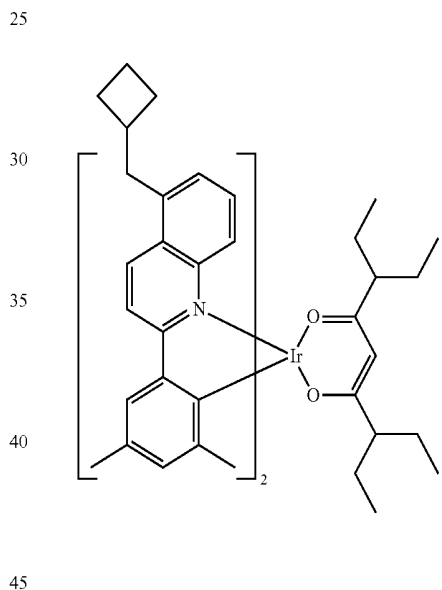
Compound II-29
