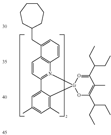
Compound II-33
