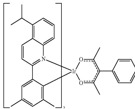
Compound 21
