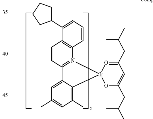
Compound II-10
