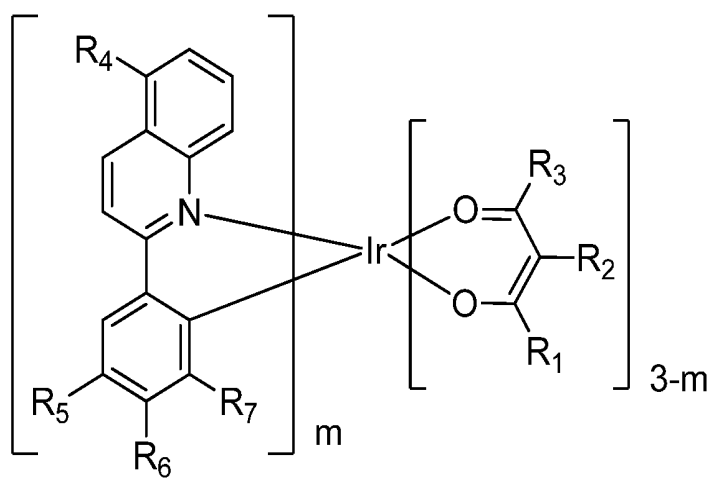
Formula III
