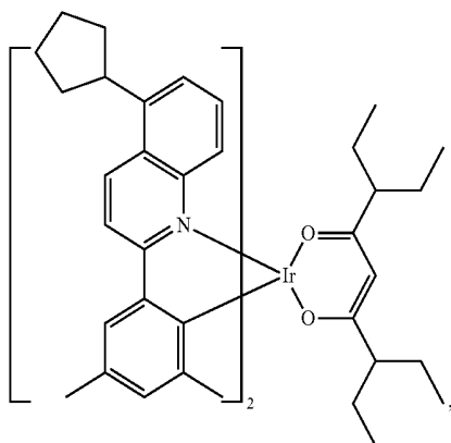
Compound II-15
