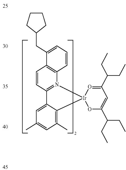
Compound II-30
