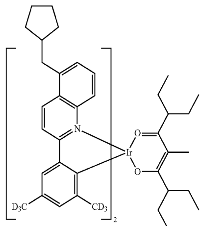
Compound II-70
