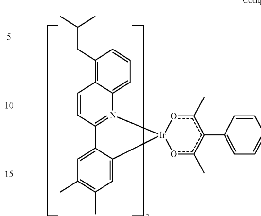
Compound 38
