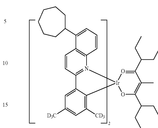
Compound II-53
