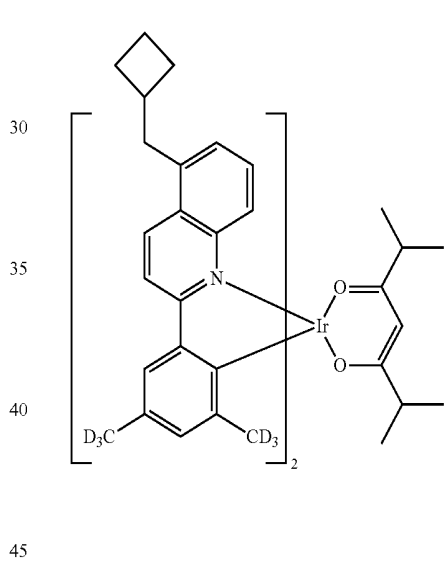
Compound II-57
