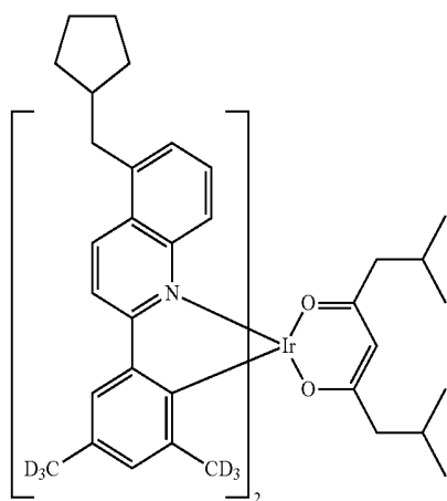
Compound II-62
