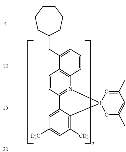
Compound II-56
