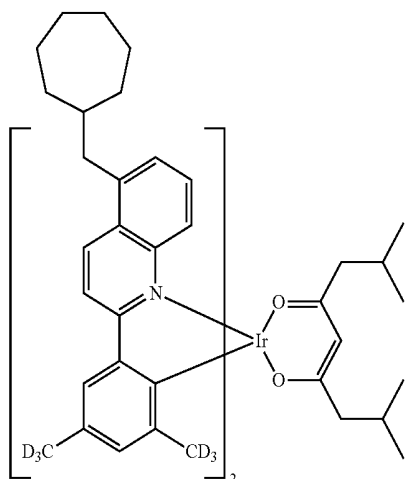
Compound II-64
