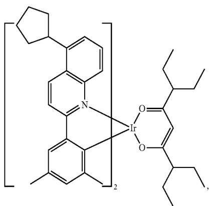
Compound II-15
