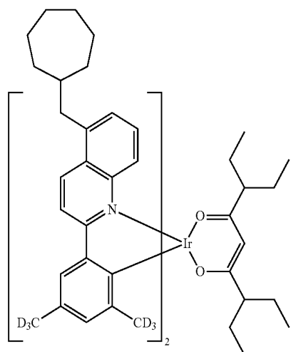
Compound II-68
