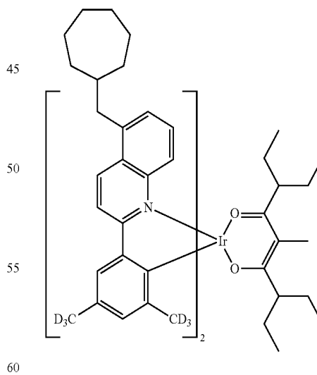
Compound II-69
