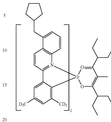
Compound II-71
