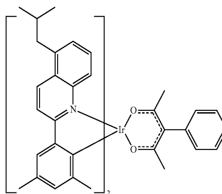
Compound 6
