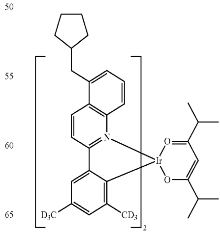
Compound II-58
