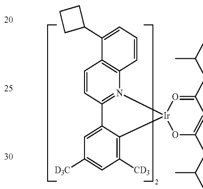
Compound II-41
