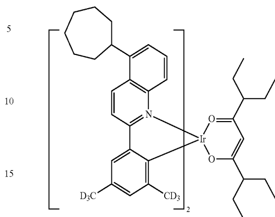
Compound II-50
