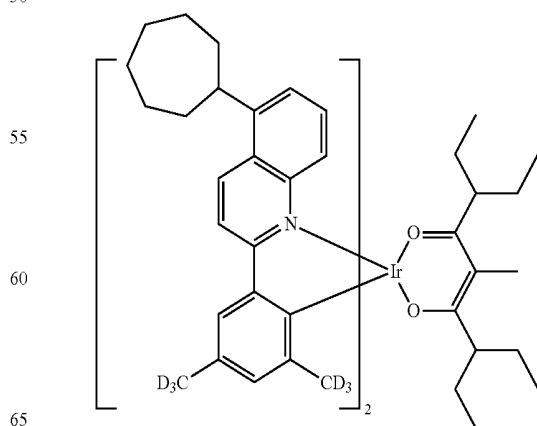
Compound II-52
