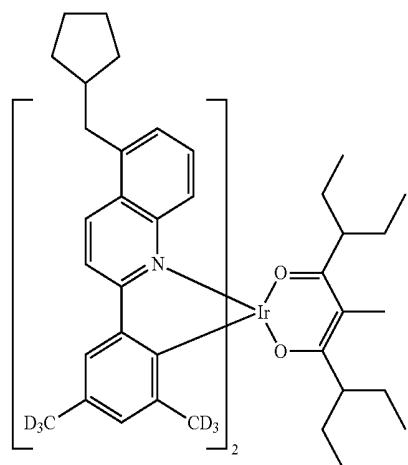
Compound II-70
