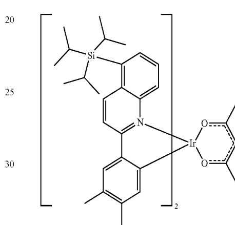
Compound 38
