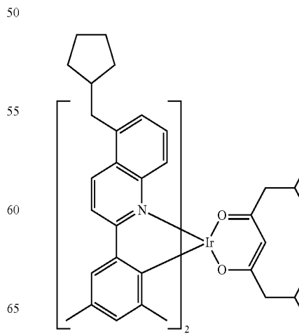
Compound II-26
