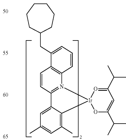
Compound II-21
