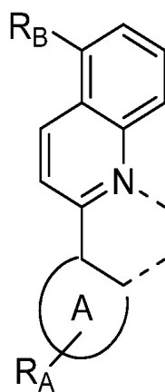
Formula I
