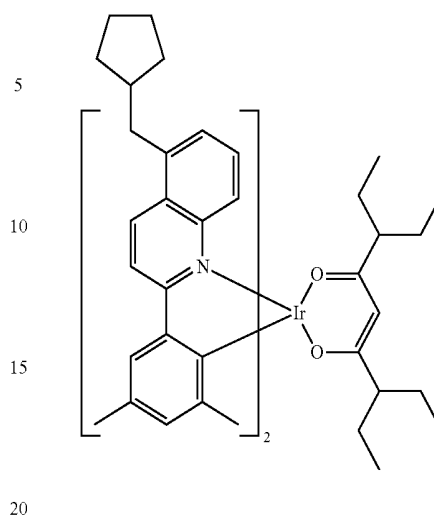
Compound II-27
