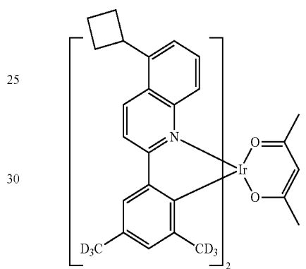
Compound II-34
