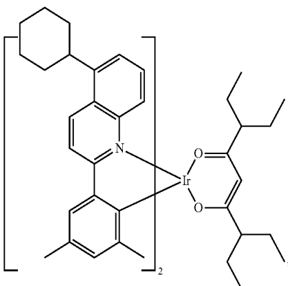
Compound II-16
