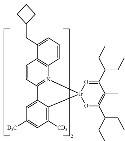
Compound II-69
