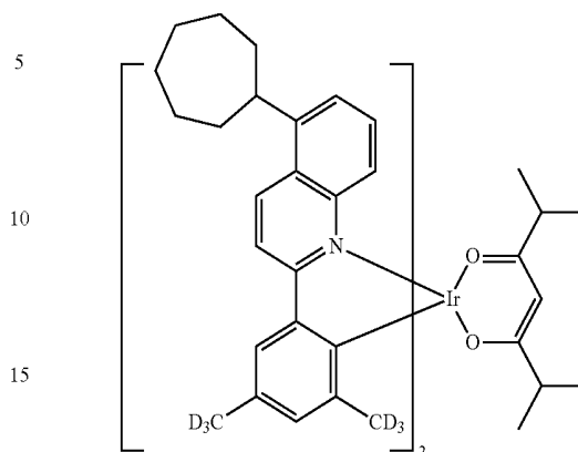
Compound II-45
